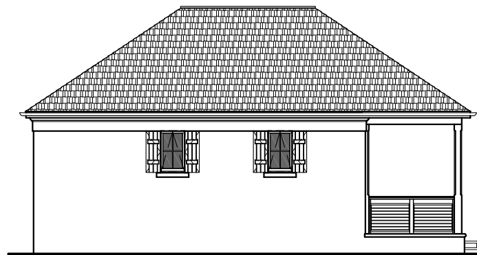
LEFT ELEVATION
